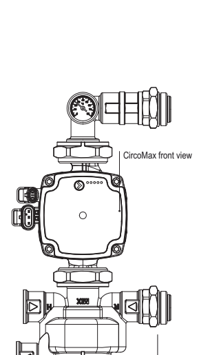
CircoMax front view
